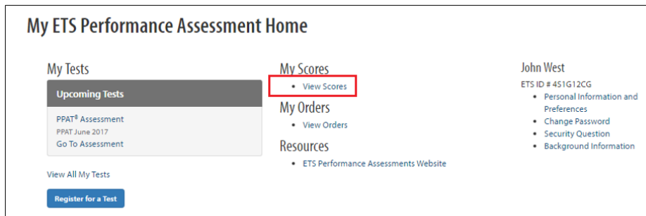
Figure 47: View Scores
